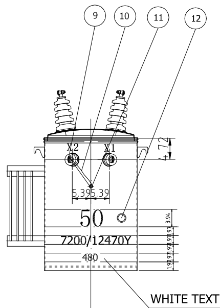
LV BUSHING TERMINAL DETAIL
